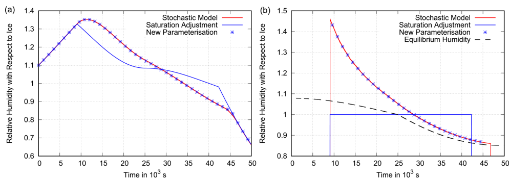
Figure 11. Scenario 2. Panel (a) shows the grid box mean relative humidity (with respect to ice) as a function of time in an updraught with an initial speed of 2 \text{ cm s}^{-1} that weakens over time and becomes a downdraught accelerating to 5 \text{ cm s}^{-1} (see Fig. 5). The assumed deposition rate is \alpha = 3 \times 10^{-4} \text{ s}^{-1} . The initial humidity distribution is narrow with a = 0.1 . The behaviour of the benchmark box model is shown in red and is closely followed by the new parameterisation (blue stars). The parameterisation that uses saturation adjustment underestimates relative humidity during the cooling period and overestimates it during the warming period more strongly due to the narrower clear-sky humidity distribution. Panel (b) presents the corresponding mean in-cloud relative humidity for the stochastic model, the new parameterisation and the parameterisation with saturation adjustment. The box model and the new parameterisation approach the equilibrium supersaturation (dashed black line), while saturation adjustment assumes exactly saturated conditions inside the cloud.
