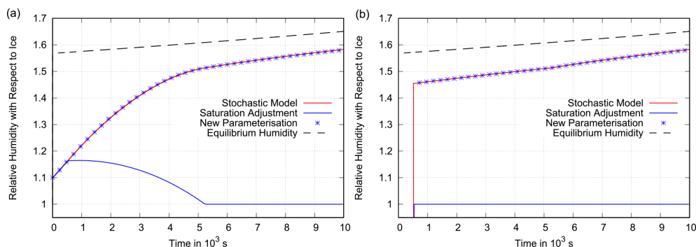
Figure 12. Scenario 1. Panel (a) shows the grid box mean relative humidity (with respect to ice) as a function of time in a fast constant updraught of 10 \text{ cm s}^{-1} . Other simulation parameters are \alpha = 3 \times 10^{-4} \text{ s}^{-1} and a = 0.25 . The behaviour of the benchmark box model is shown in red. It increases steadily and is closely followed by the new parameterisation (blue stars), while the parameterisation that uses saturation adjustment does not even reproduce the same trend. Hence, in principle, the new parameterisation is capable of simulating large supersaturations beyond the threshold for homogeneous nucleation occasionally found in the real atmosphere. However, the box model result quickly becomes unrealistic, as the increasing supersaturation would cause \alpha to grow due to a rapid increase in crystal number density. Panel (b) presents the corresponding mean in-cloud relative humidity for the stochastic model, the new parameterisation and the parameterisation with saturation adjustment. The box model and the new parameterisation approach the equilibrium supersaturation (dashed black line), while saturation adjustment assumes exactly saturated conditions inside the cloud.
