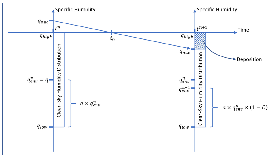
Figure 3. Schematic on the initiation of cloud formation in the parameterisation. At the time t_0 , q_{\text{nuc}} propagates into the clear-sky humidity distribution, thereby causing nucleation in the moistest part of the grid box. The parameterisation turns this part into a cloud, and q_{\text{nuc}} becomes the new top of the clear-sky humidity distribution. The mean clear-sky humidity q_{\text{env}} is adjusted accordingly.
