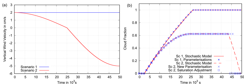
Figure 5. Panel (a) presents a visualisation of the considered vertical wind speed scenarios. Scenario 1 is characterised by a constant updraught, whereas the vertical wind speed in Scenario 2 follows half a period of a cosine function in time with an increase in amplitude halfway through the simulation from 2 to 5 \text{cm s}^{-1} . Panel (b) shows the corresponding evolutions of the cloud fraction in the stochastic model and the parameterisations for \alpha = 3 \times 10^{-4} \text{ s}^{-1} and a = 0.25 . As can be seen, the parameterisations both capture the evolution of the cloud fraction precisely. Only the process of cloud dissolution is not modelled accurately, as the cloud fraction is simply set to zero once all ice has sublimated. Note that the sublimation process is slower in the new parameterisation compared with the one using saturation adjustment, thereby increasing the cloud lifetime.
