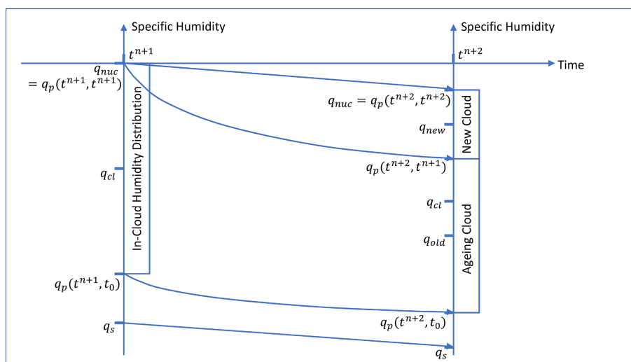
Figure 4. Schematic of the evolution of the in-cloud humidity during ongoing cloud formation. The boundaries of the humidity distribution in the already existing cloud decay exponentially towards q_s , while the steady decrease in q_{nuc} continuously causes nucleation in further parts of the clear-sky portion of the grid box. These new cloud parts begin their own decay towards q_s at their individual nucleation times, resulting in a steady new humidity distribution in the grown cloud with the new q_{nuc} as its top end.
