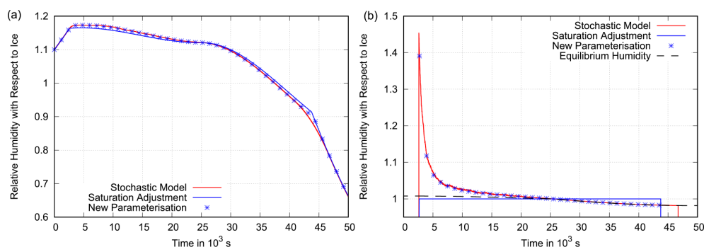
Figure 9. Scenario 2. Panel (a) shows the grid box mean relative humidity (with respect to ice) as a function of time with a = 0.25 in an updraught with an initial speed of 2 \text{ cm s}^{-1} that weakens over time and becomes a downdraught accelerating to 5 \text{ cm s}^{-1} (see Fig. 5). The assumed deposition rate is high, \alpha = 2.8 \times 10^{-3} \text{ s}^{-1} , which corresponds to a cloud with 1000 crystals of 10 \mu\text{m} radius per litre. The behaviour of the benchmark box model is shown in red and is closely followed by the new parameterisation (blue stars). The parameterisation that uses saturation adjustment only slightly underestimates relative humidity during the cooling period and slightly overestimates it during the warming period due to the large deposition rate. Panel (b) presents the corresponding mean in-cloud relative humidity for the stochastic model, the new parameterisation and the parameterisation with saturation adjustment. The box model and the new parameterisation approach the equilibrium supersaturation (dashed black line), while saturation adjustment assumes exactly saturated conditions inside the cloud.
