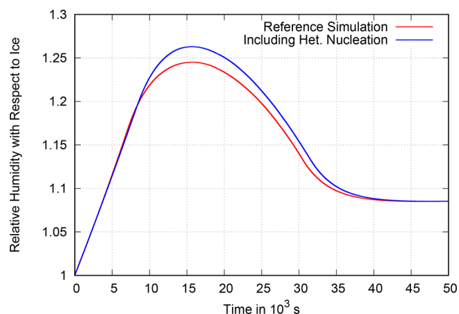
Figure 17. Evolution of the grid box mean relative humidity in the stochastic box model in a simulation with a second nucleation threshold at 130 % representing heterogeneous nucleation (blue). For each air parcel, \alpha is set to 1.5 \times 10^{-5} \text{ s}^{-1} once its relative humidity exceeds 130 % and to 3 \times 10^{-4} \text{ s}^{-1} once it exceeds the threshold for homogeneous nucleation. The red curve shows the reference simulation of the stochastic box model from Fig. 6 with constant \alpha = 3 \times 10^{-4} \text{ s}^{-1} but starting from 100 % relative humidity. The heterogeneously induced deposition removes vapour from the moistest air parcels, thereby delaying the onset of homogeneous nucleation. This leads to an overall increase in the grid box mean relative humidity.
