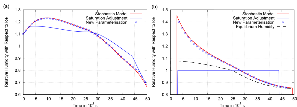
Figure 14. Scenario 2. Panel (a) shows the grid box mean relative humidity (with respect to ice) as a function of time in an updraught with an initial speed of 2 \text{ cm s}^{-1} that weakens over time and becomes a downdraught accelerating to 5 \text{ cm s}^{-1} (see Fig. 5). Other simulation parameters are \alpha = 3 \times 10^{-4} \text{ s}^{-1} and a = 0.25 . The time step of the parameterisations is increased to 10 min. The behaviour of the benchmark box model is shown in red and is still closely followed by the new parameterisation (blue stars). The parameterisation that uses saturation adjustment underestimates relative humidity during the cooling period and overestimates it during the warming period. Panel (b) presents the corresponding mean in-cloud relative humidity for the stochastic model, the new parameterisation and the parameterisation with saturation adjustment. The box model and the new parameterisation approach the equilibrium supersaturation (dashed black line), while saturation adjustment assumes exactly saturated conditions inside the cloud.
