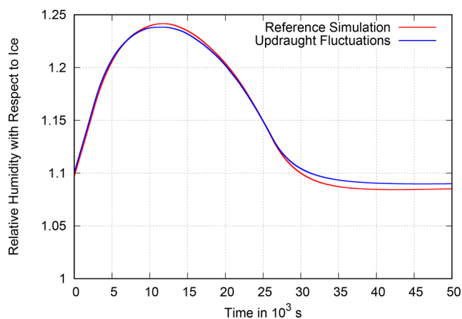
Figure 15. Evolution of the grid box mean relative humidity in the stochastic box model in a simulation in which each air parcel experiences a random updraught of between 1 and 3 cm s −1 (blue) every time step. \alpha varies with the updraught velocity at the time of nucleation in the individual air parcel around \alpha_0 = 3 \times 10^{-4} \text{ s}^{-1} . The red plot shows the reference simulation of the stochastic box model from Fig. 6 with uniform w = 2 \text{ cm s}^{-1} and uniform \alpha = 3 \times 10^{-4} \text{ s}^{-1} for all air parcels. Even though the updraught fluctuations cause a slightly larger mean value of \alpha , they lead to an increased equilibrium humidity in the aged cloud due to the non-linear dependence of S_{\text{eq}} on \frac{d \ln(q_s)}{dt} .
