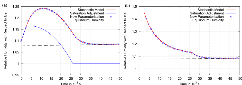
Figure 6. Scenario 1. Panel (a) shows the grid box mean relative humidity (with respect to ice) as a function of time in a grid box with a = 0.25 that undergoes cooling in a constant updraught of 2 \text{ cm s}^{-1} and cloud formation with \alpha = 3 \times 10^{-4} \text{ s}^{-1} . Shown is the behaviour of the stochastic box model that treats one grid box as an ensemble of 10^4 air parcels with an initial distribution of specific humidity (red line); this model is assumed to best represent reality and serves as a benchmark for the parameterisations. The new parameterisation (blue stars) follows the stochastic model closely, while the parameterisation that uses saturation adjustment does not, leading to an underestimation of the mean relative humidity and, thus, of supersaturation. The new parameterisation approaches the equilibrium supersaturation (dashed black line), while saturation adjustment assumes exactly saturated conditions inside the cloud. Panel (b) presents the corresponding mean in-cloud relative humidity for the stochastic model, the new parameterisation and the parameterisation with saturation adjustment. One can clearly see how the decay of humidity in the stochastic box model changes into a pure exponential decay once the cloud fraction reaches unity and no new, highly supersaturated cloud parts join the cloud anymore (see Fig. 5b).
