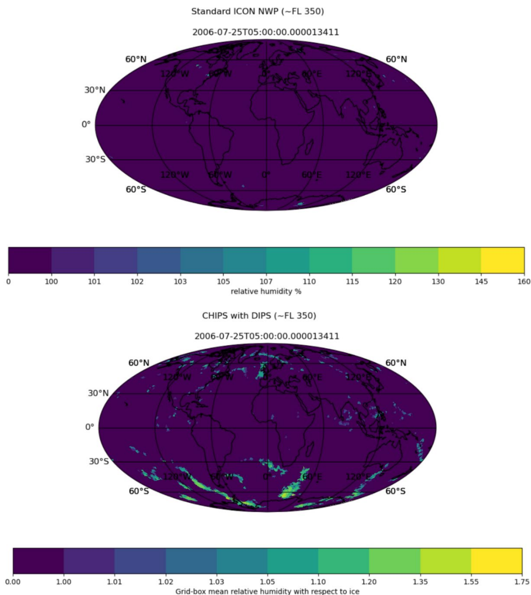
Figure: Test of the new one-moment cloud physics in a course resolution ICON simulation. Top panel: the original ICON cloud physics does hardly produce any ice supersaturation. Bottom panel: in contrast, the new DIPS-physics parameterization shows some ice supersaturation (blue and green patches).
