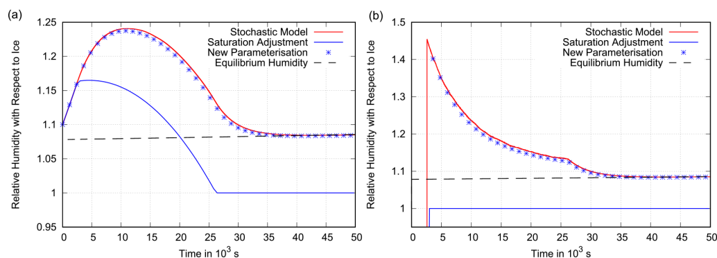
Figure 13. Scenario 1. Panel (a) shows the grid box mean relative humidity (with respect to ice) as a function of time in a constant updraught of 2 \text{ cm s}^{-1} . Other simulation parameters are \alpha = 3 \times 10^{-4} \text{ s}^{-1} and a = 0.25 . The time step of the parameterisations is increased to 10 min. The behaviour of the benchmark box model is shown in red. The new parameterisation (blue stars) still follows the benchmark simulation quite closely, while the parameterisation that uses saturation adjustment does not, leading to an underestimation of relative humidity. Panel (b) presents the corresponding mean in-cloud relative humidity for the stochastic model, the new parameterisation and the parameterisation with saturation adjustment. The box model and the new parameterisation approach the equilibrium supersaturation (dashed black line), while saturation adjustment assumes exactly saturation inside the cloud.
