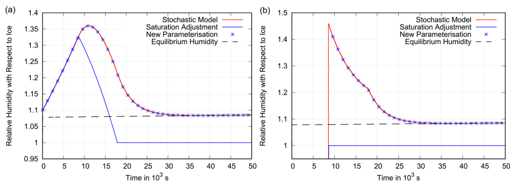
Figure 10. Scenario 1. Panel (a) shows the grid box mean relative humidity (with respect to ice) as a function of time in a constant updraught of 2 \text{ cm s}^{-1} . The assumed deposition rate is \alpha = 3 \times 10^{-4} \text{ s}^{-1} . The initial humidity distribution is narrow with a = 0.1 . The behaviour of the benchmark box model is shown in red. The new parameterisation (blue stars) follows the benchmark simulation closely, while the parameterisation that uses saturation adjustment does not, leading to a larger underestimation of relative humidity compared with the reference simulation in Fig. 6. Panel (b) presents the corresponding mean in-cloud relative humidity for the stochastic model, the new parameterisation and the parameterisation with saturation adjustment. The box model and the new parameterisation approach the equilibrium supersaturation (dashed black line), while saturation adjustment assumes exactly saturation inside the cloud.
