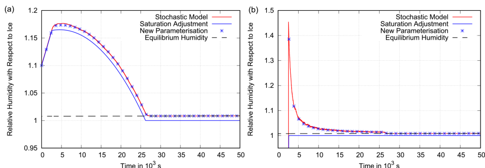
Figure 8. Scenario 1. Panel (a) shows the grid box mean relative humidity (with respect to ice) as a function of time in a constant updraught of 2 \text{ cm s}^{-1} with a = 0.25 . The assumed deposition rate is high, \alpha = 2.8 \times 10^{-3} \text{ s}^{-1} , which corresponds to a cloud with 1000 crystals of 10 \mu\text{m} radius per litre. The behaviour of the benchmark box model is shown in red. The new parameterisation (blue stars) follows the benchmark simulation closely, while the parameterisation that uses saturation adjustment does not. This leads to only a slight underestimation of relative humidity due to the large deposition rate. Panel (b) presents the corresponding mean in-cloud relative humidity for the stochastic model, the new parameterisation and the parameterisation with saturation adjustment. The box model and the new parameterisation approach the equilibrium supersaturation (dashed black line), while saturation adjustment assumes exactly saturation inside the cloud.
