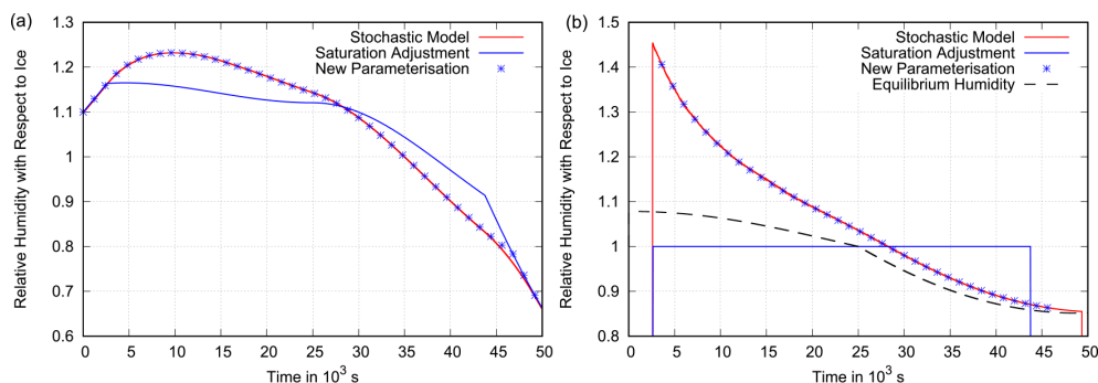
Figure 7. Scenario 2. Panel (a) shows the grid box mean relative humidity (with respect to ice) as a function of time in an updraught with an initial speed of 2 \text{ cm s}^{-1} that weakens over time and becomes a downdraught accelerating to 5 \text{ cm s}^{-1} (see Fig. 5). Other simulation parameters are \alpha = 3 \times 10^{-4} \text{ s}^{-1} and a = 0.25 . The behaviour of the benchmark box model is shown in red. The new parameterisation (blue stars) follows the benchmark simulation closely, while the parameterisation that uses saturation adjustment does not, leading to an underestimation of relative humidity during the cooling period and an overestimation during the warming period. Panel (b) presents the corresponding mean in-cloud relative humidity for the stochastic model, the new parameterisation and the parameterisation with saturation adjustment. The box model and the new parameterisation approach the equilibrium supersaturation (dashed black line), while saturation adjustment assumes exactly saturated conditions inside the cloud.
