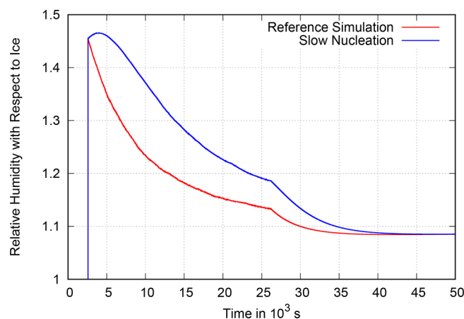
Figure 16. Evolution of the in-cloud mean relative humidity in the stochastic box model in a simulation in which \alpha starts at zero at the onset of nucleation in every air parcel and increases over time to \alpha = 3 \times 10^{-4} \text{ s}^{-1} (blue) compared with the reference simulation of the stochastic box model from Fig. 6 with constant \alpha = 3 \times 10^{-4} \text{ s}^{-1} (red). Accounting for the phase of initial crystal growth leads to a short further increase in supersaturation after the onset of nucleation before deposition becomes fast enough to deplete the supersaturation, resulting in a considerable delay in the relaxation process.
